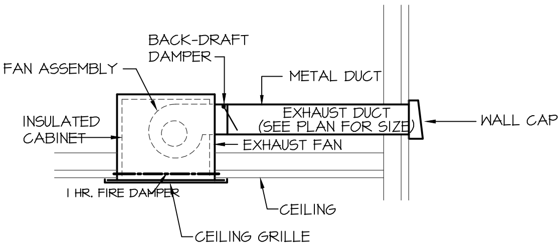
CEILING MOUNTED EXHAUST FAN DETAIL NO SCALE
