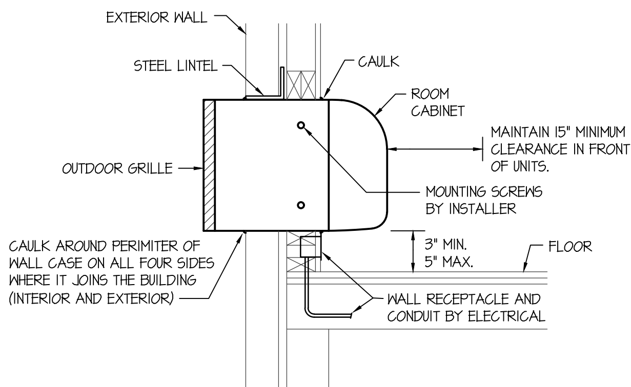
THRU-THE-WALL A/C UNIT DETAIL NO SCALE
